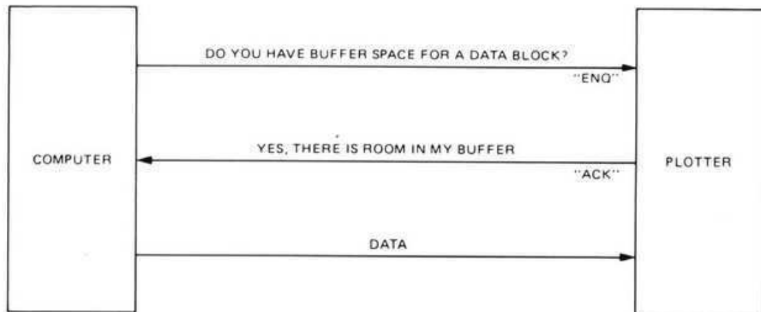
ENQ/ACK Handshake Protocol Example 1
