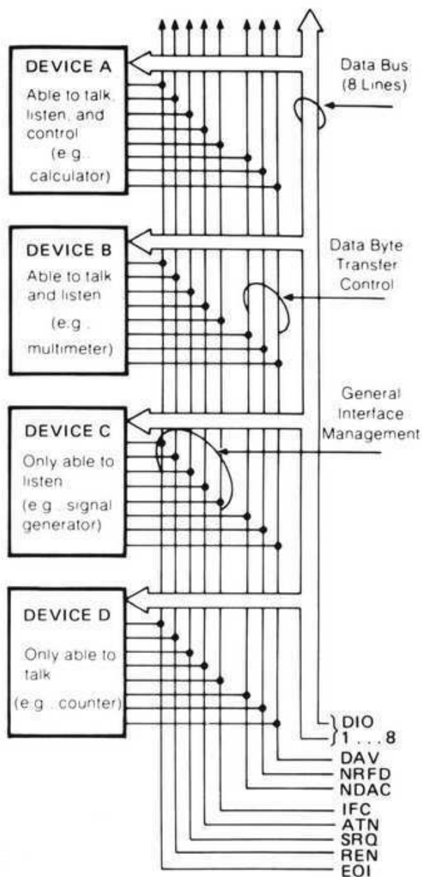
HP-IB Signal Lines
