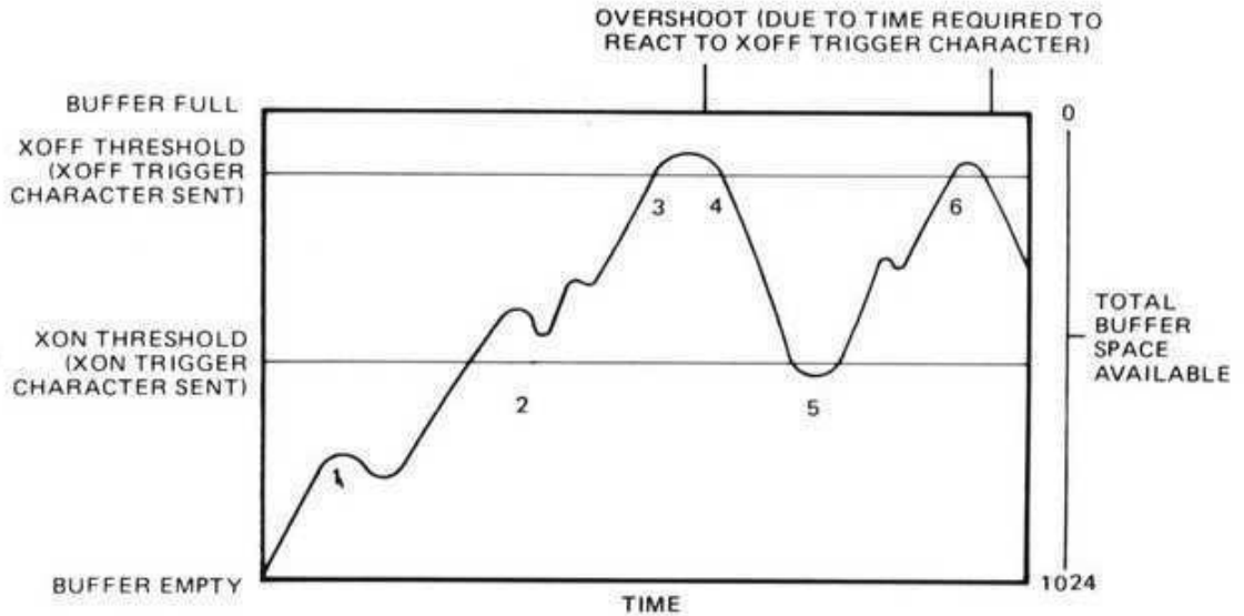
Xon-Xoff Threshold Levels
