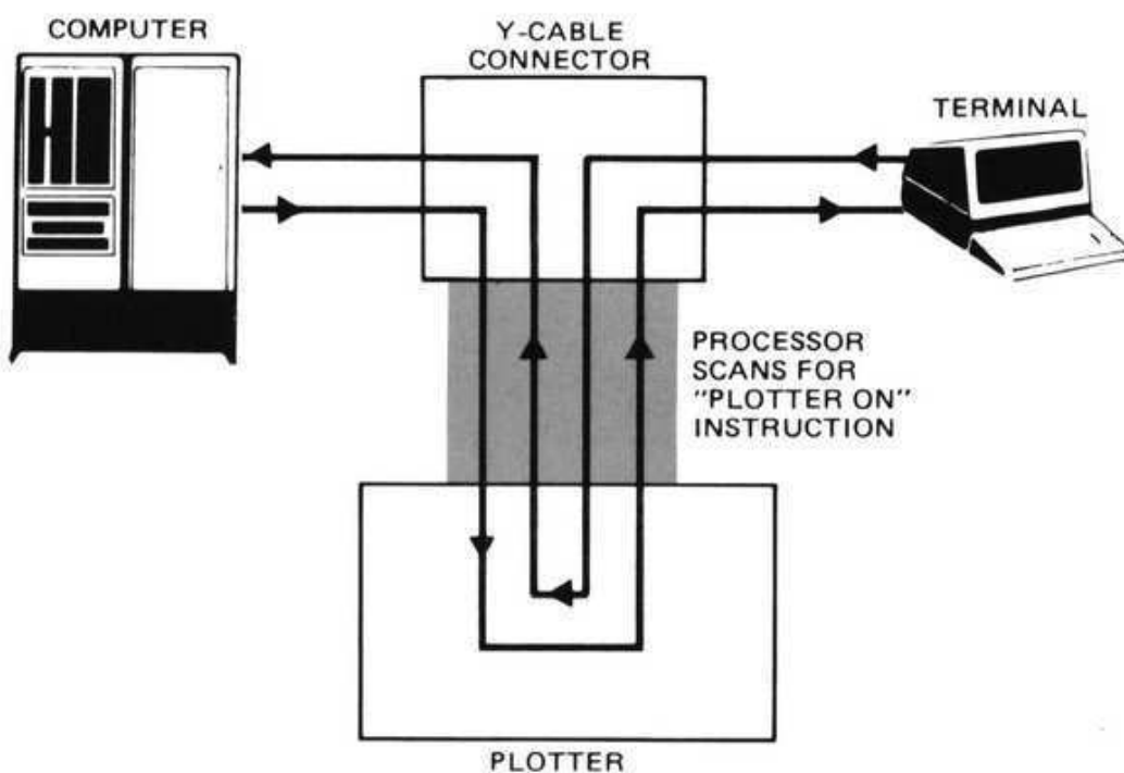
Plotter in On-Line, Programmed-Off State
