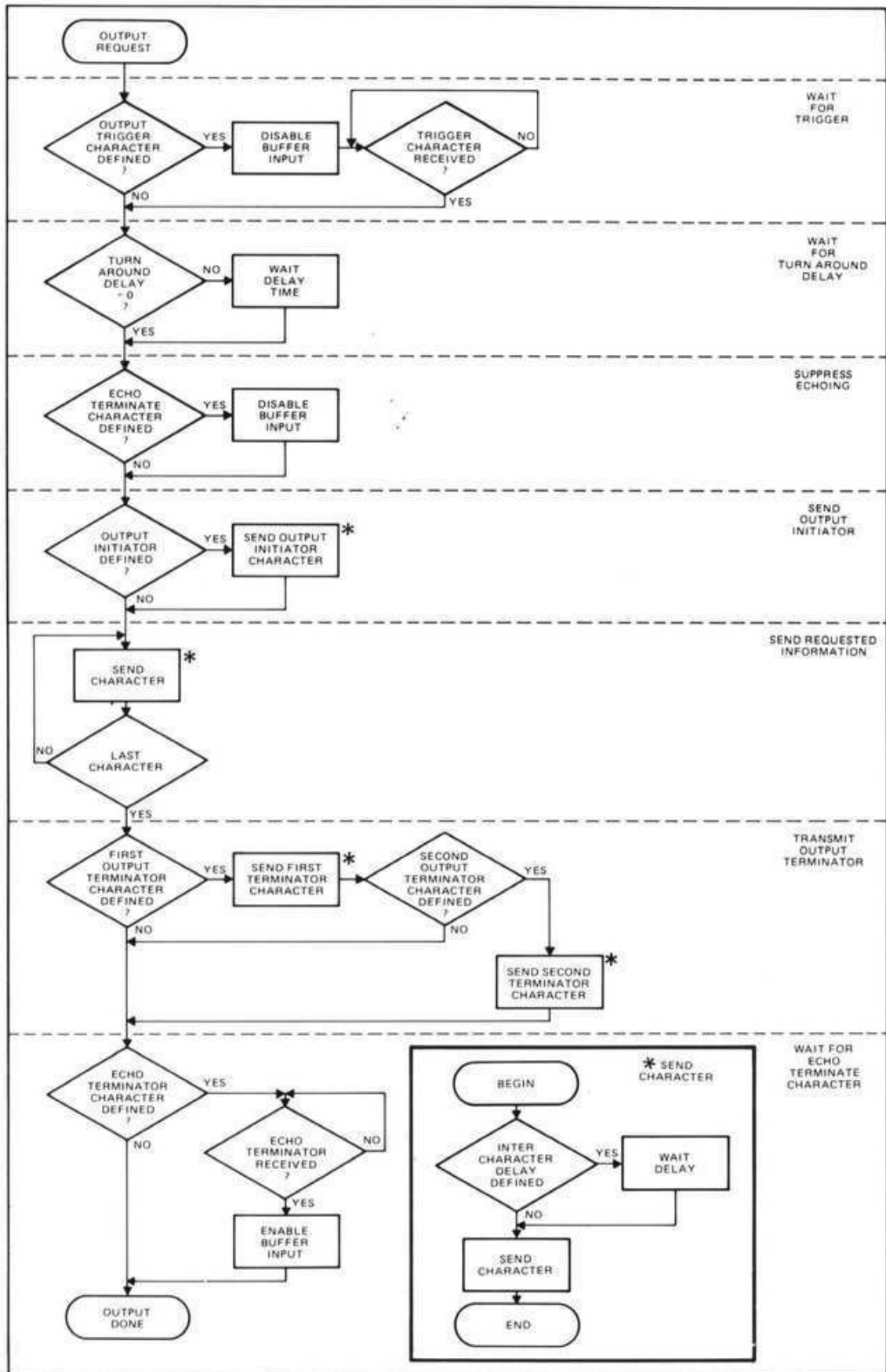
Output Request Flow Chart
