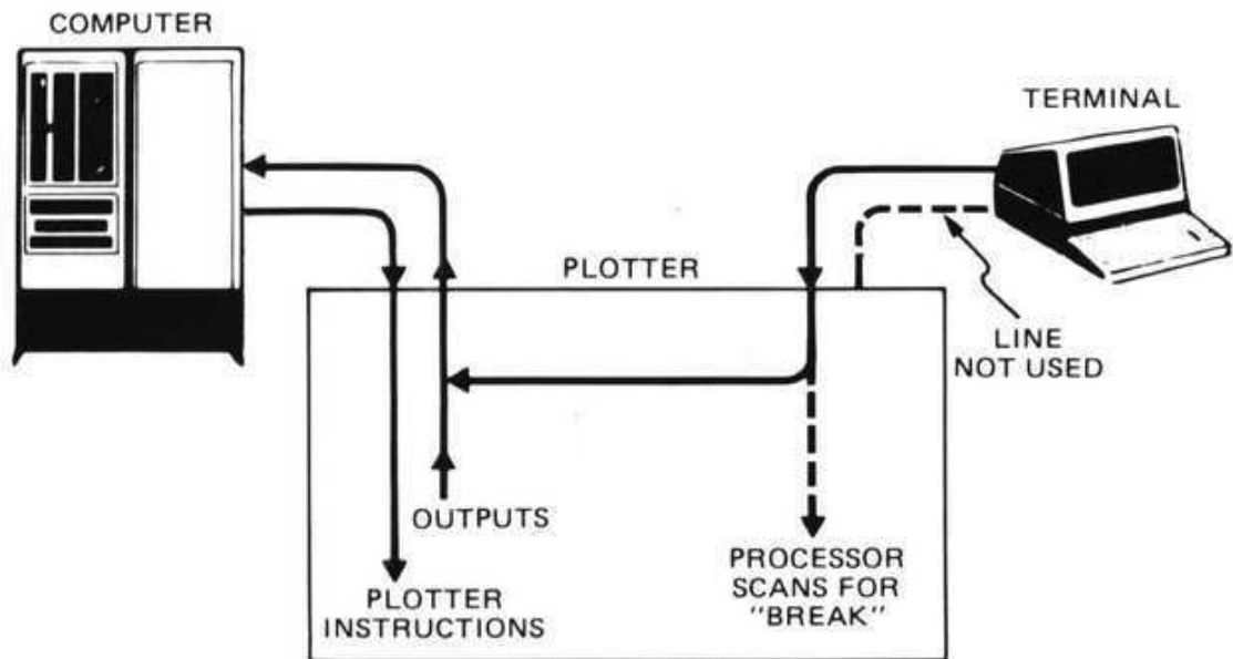
Plotter in On-Line, Programmed-On State
