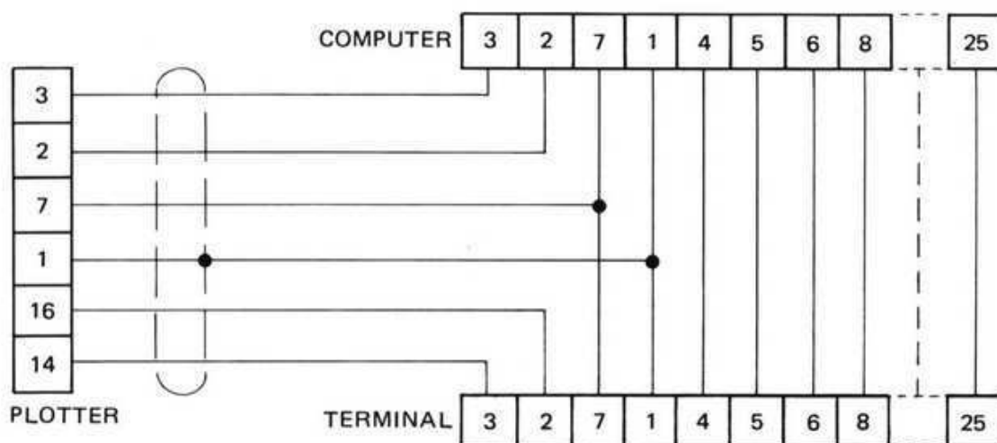
Y-cable Schematic
