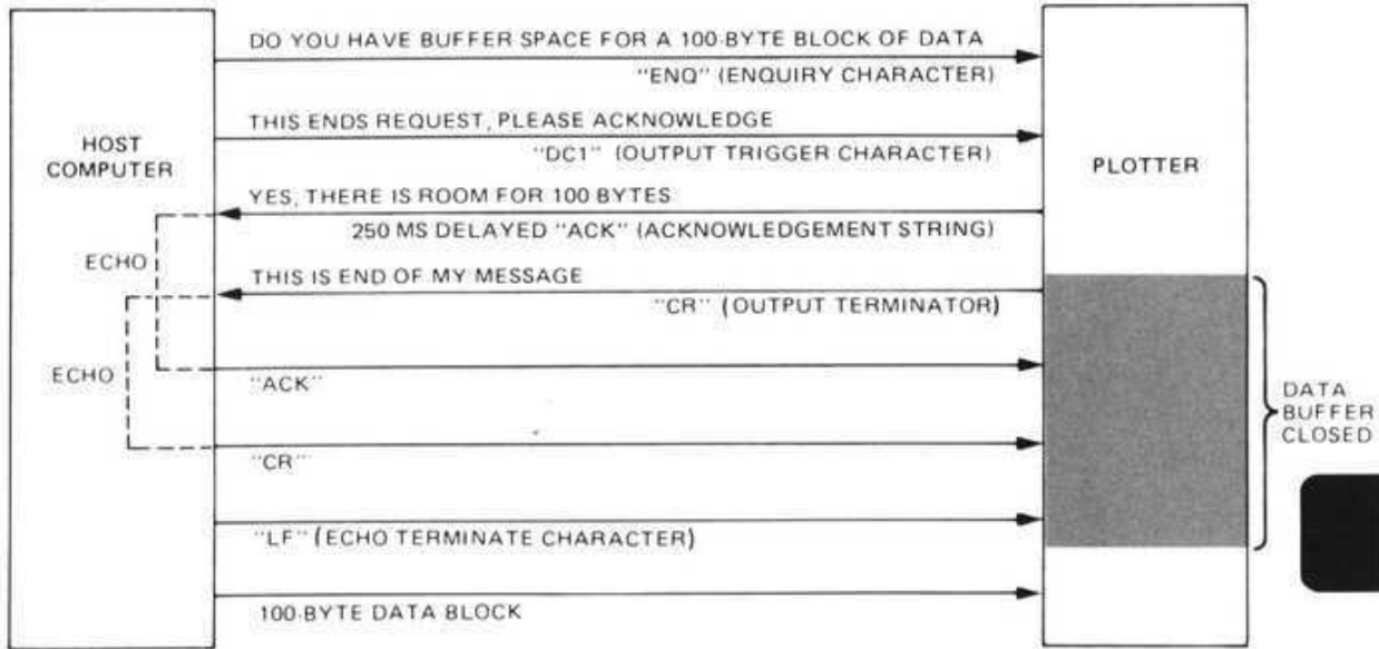
ENQ/ACK Handshake Protocol Example 2
