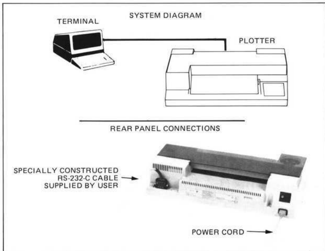
Plotter Interconnection with Only a Terminal
